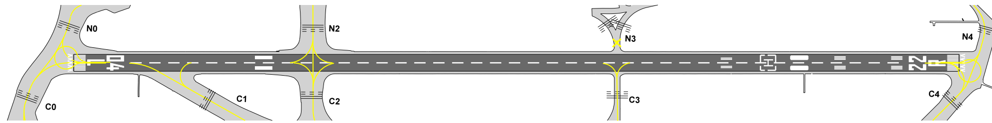
MARKING AIDS RWY 04L / 22R AND EXIT TWY
