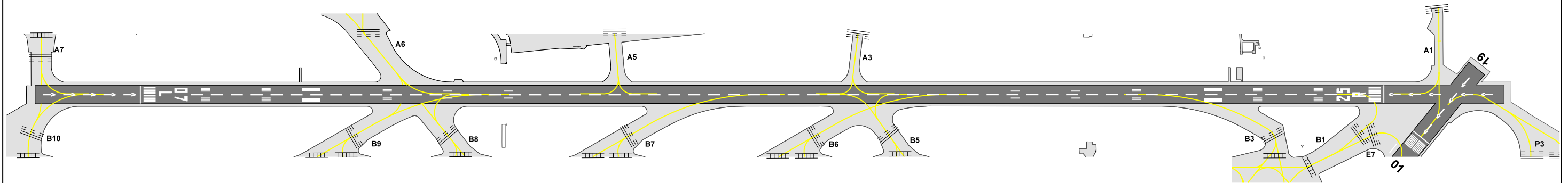
MARKING AIDS RWY 07R / 25L AND EXIT TWY
